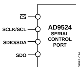
Figure 36. Serial Control Port
