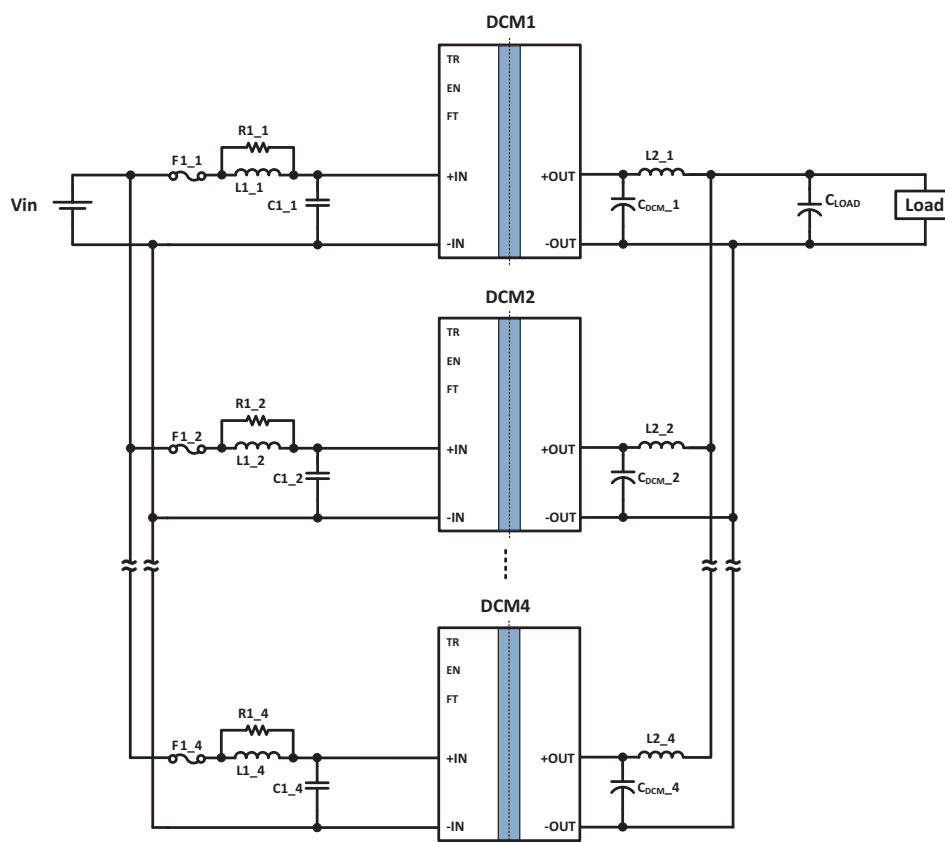
Typical Application 1: MDCM28AP480M320A50 in an array of four units
