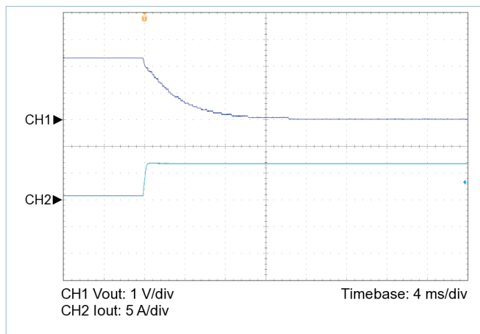
Figure 8 — 10% to 100% load transient response, V_{IN} = 28\text{ V} , nominal trim, C_{OUT\_EXT} = 200\text{ }\mu\text{F}
