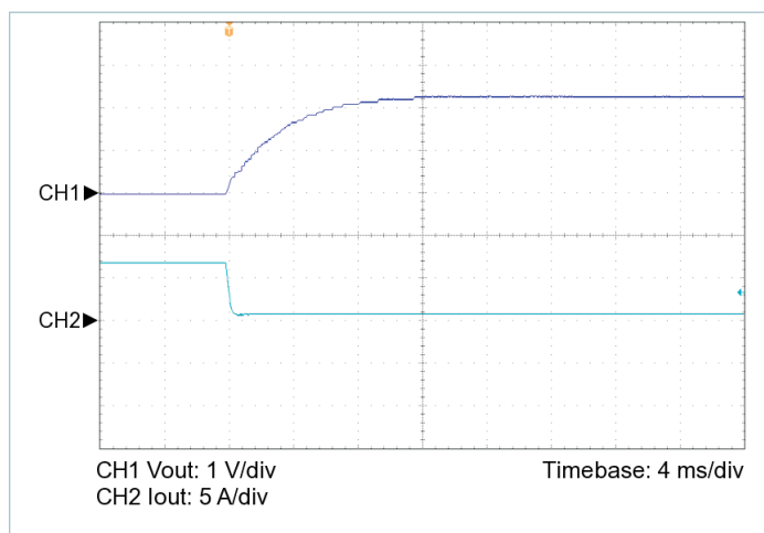
Figure 7 — 100% to 10% load transient response, V_{IN} = 28\text{ V} , nominal trim, C_{OUT\_EXT} = 200\text{ }\mu\text{F}
