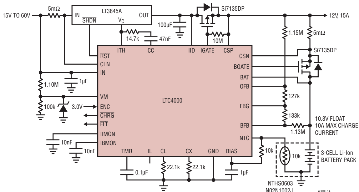
Figure 14. 48V to 10.8V at 10A Buck Converter Charger for Three LiFePO 4 Cells
