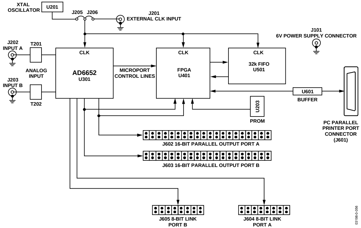
Figure 65. Simplified Block Diagram of AD6652 PCB
