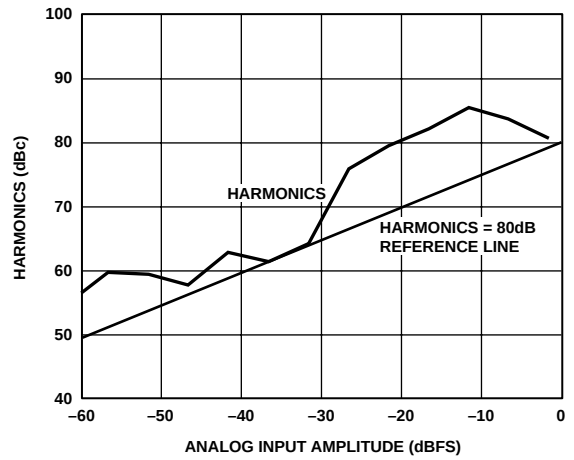
Figure 13. Harmonics vs. Analog Amplitude at 68 MHz
