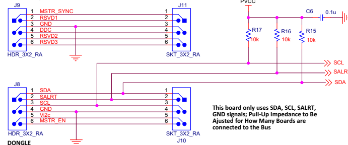
FIGURE 7. I/O CONNECTORS, AUXILIARY CIRCUITS AND ON-BOARD TRANSIENT LOAD SCHEMATICS
