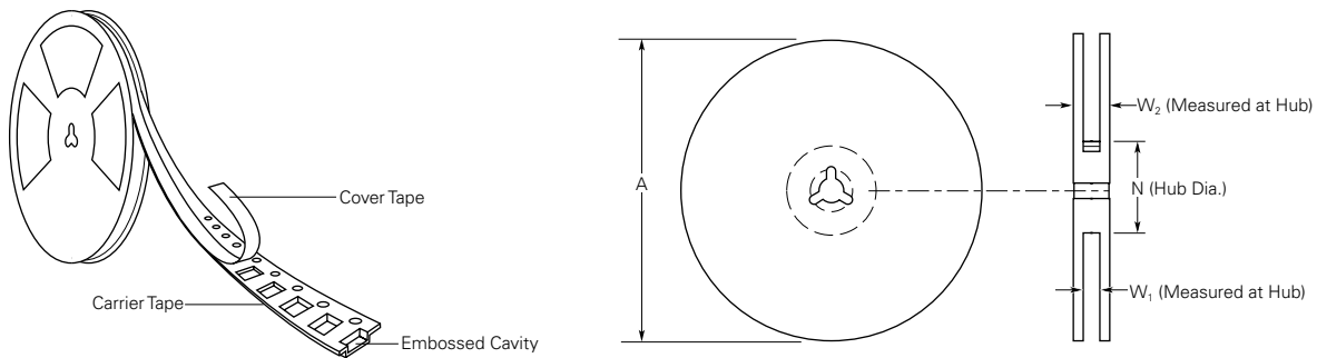
Figure A30 — EIA Referenced Reel Dimensions for AHS/ASMD/femtoASMDC/picoASMDC/nanoASMDC/microASMD/miniASMDC/ASMDC/nanoASMDC PolySwitch Automotive Devices
