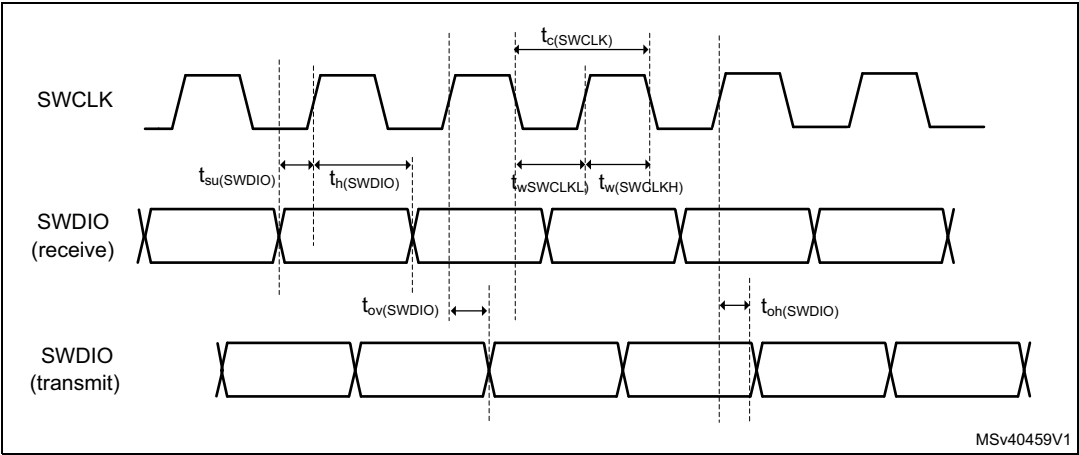
Figure 63. SWD timing
