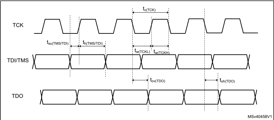
Figure 62. JTAG timing diagram
