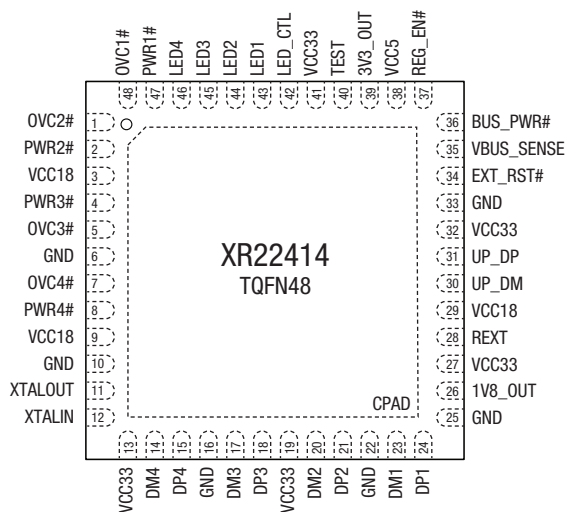
Top View, TQFN48
