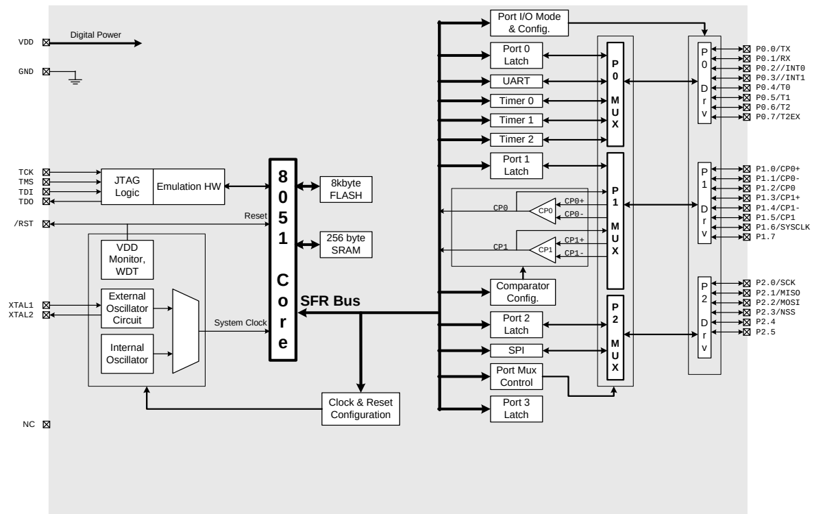
Figure 1.4. C8051F231 Block Diagram (32 LQFP)
