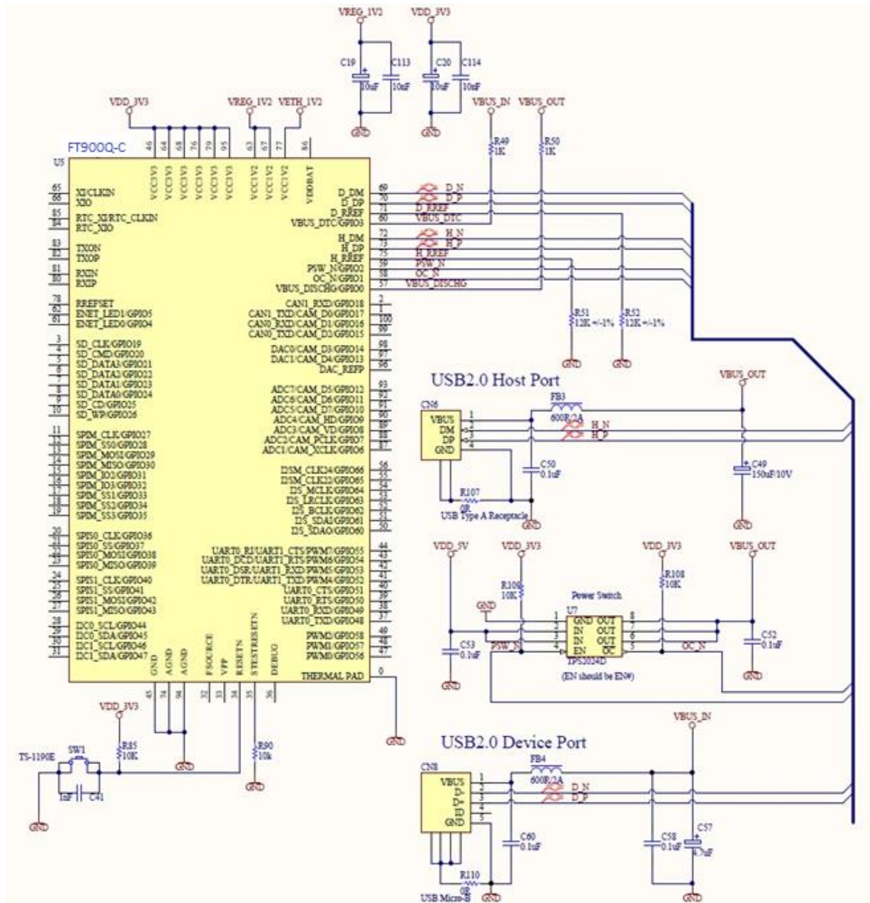
Figure 4-6 – USB Connectors
