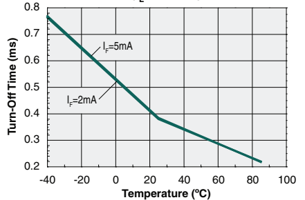
Typical Turn-Off Time vs. Temperature (I L =100mA)
