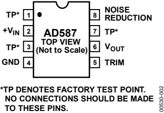
Figure 2. Pin Configuration
