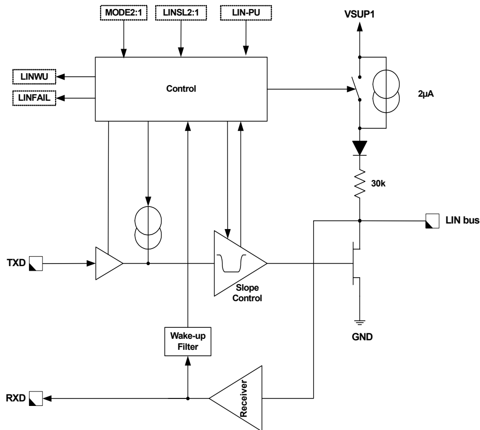
Figure 15. LIN Interface
