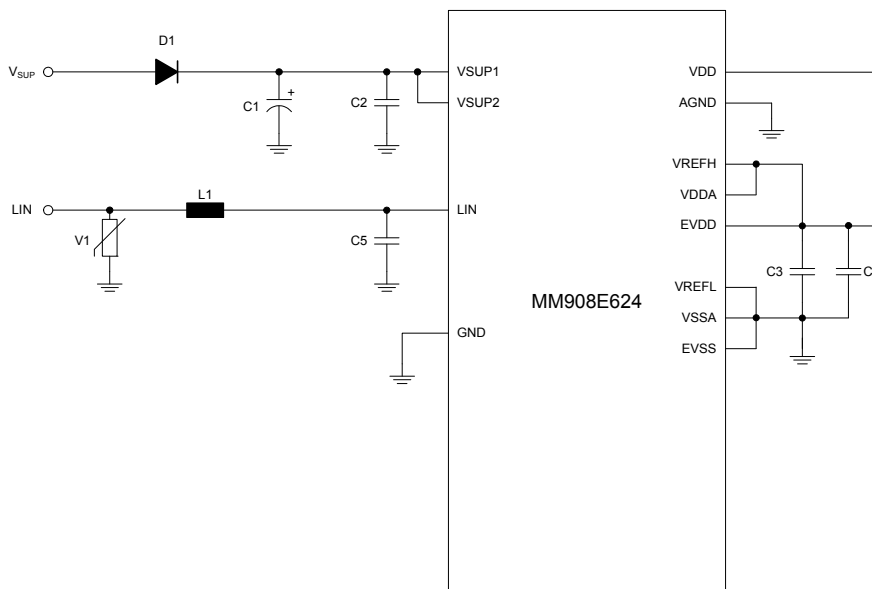
Figure 20. EMC/EMI Recommendations
