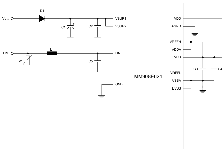
Figure 20. EMC/EMI Recommendations
