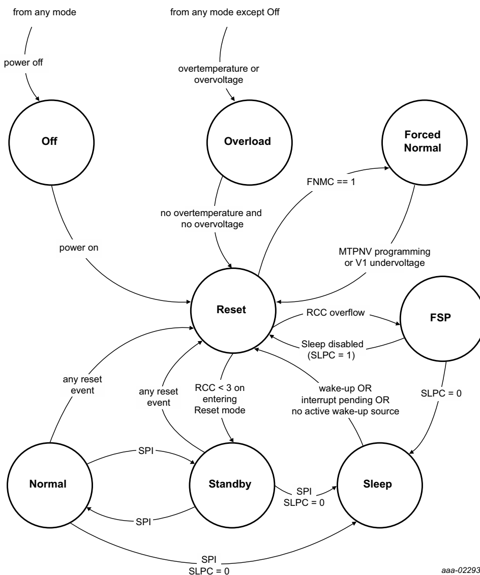
Fig 4. UJA113x system controller
