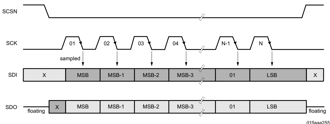
Fig 23. SPI timing protocol
