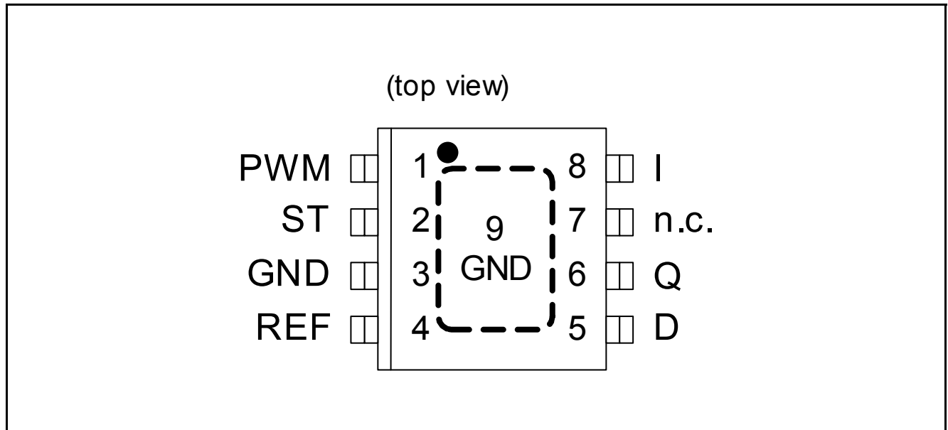
Figure 3-1 Pin Configuration
