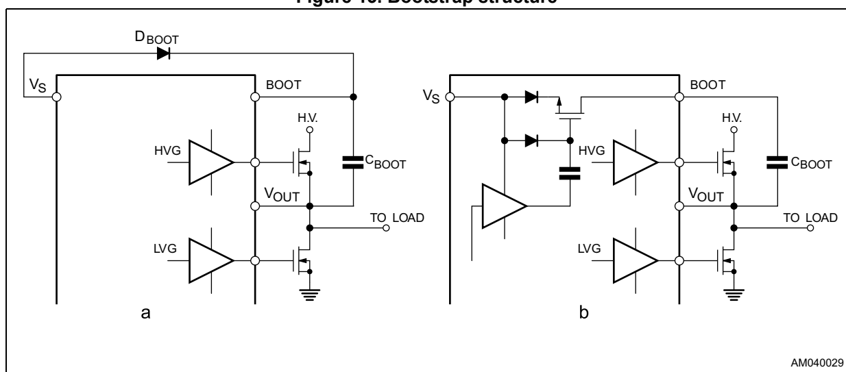
Figure 13. Bootstrap structure
