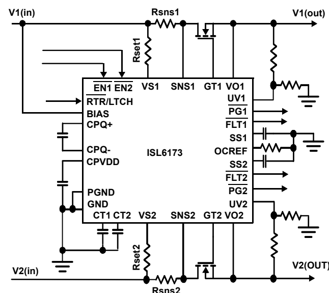
FIGURE 1. TYPICAL APPLICATION
