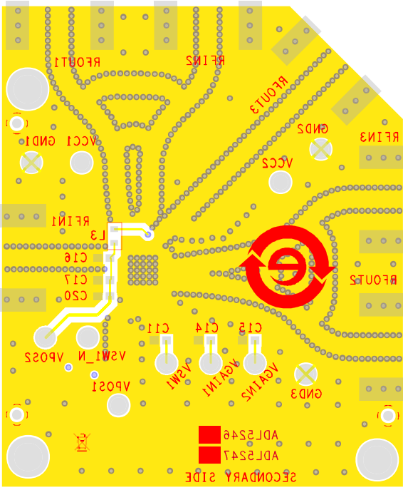
Figure 84. Evaluation Board Layout Bottom
