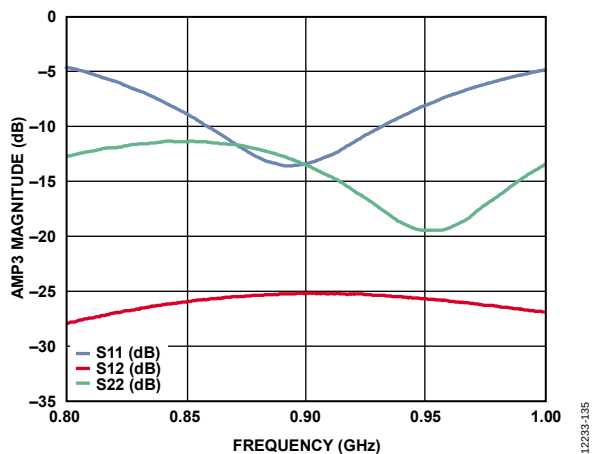
Figure 35. AMP3 0.9 GHz Input Return Loss (S11), Output Return Loss (S22), and Reverse Isolation (S12) vs. Frequency
