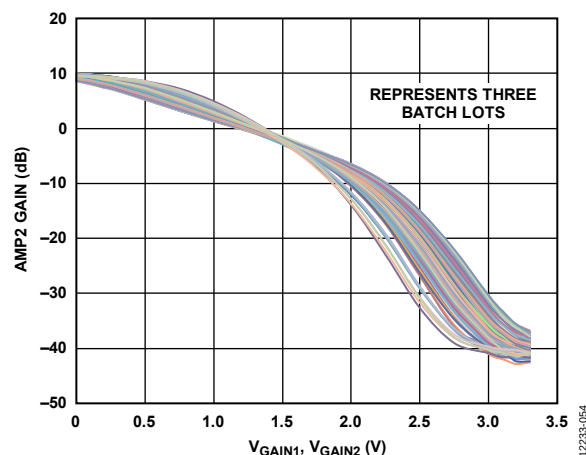
Figure 72. Distribution of AMP2 Gain vs. V_{GAIN1} , V_{GAIN2} at 1.5 GHz, 5 V Supply, HG, Both Gain Controls Varied, V_{GAIN1} = V_{GAIN2}
