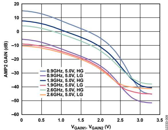
Figure 9. AMP2 Gain vs. V_{\text{GAIN1}} , V_{\text{GAIN2}} at Three Frequencies, 5 V Supply, Both Gain Controls Varied, V_{\text{GAIN1}} = V_{\text{GAIN2}}
