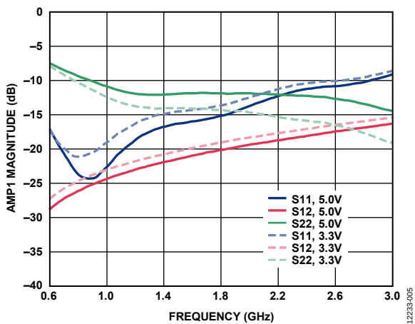
Figure 5. AMP1 Magnitude of Input Return Loss (S11), Output Return Loss (S22), and Reverse Isolation (S12) vs. Frequency
