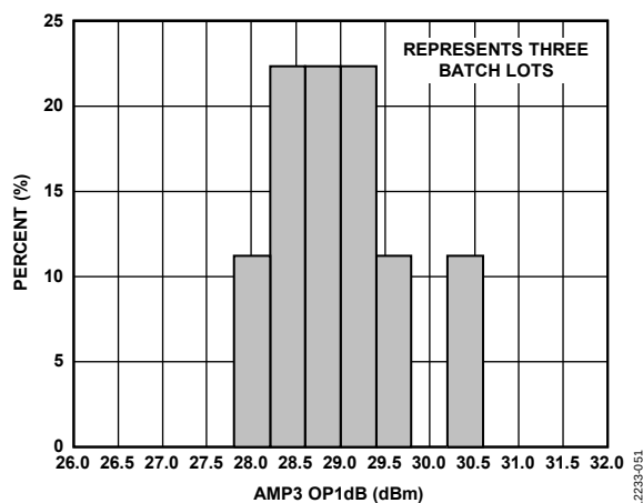
Figure 69. AMP3 OP1dB Distribution, 2.2 GHz
