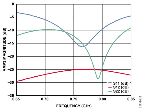
Figure 29. AMP3 0.75 GHz Magnitude of Input Return Loss (S11), Output Return Loss (S22), and Reverse Isolation (S12) vs. Frequency
