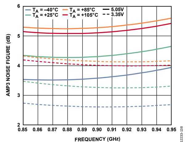
Figure 38. AMP3 0.9 GHz Noise Figure vs. Frequency by Temperature
