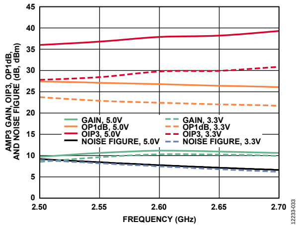
Figure 51. AMP3 2.6 GHz Gain, OIP3 at P_{OUT} = 0 dBm/Tone, OP1dB, and Noise Figure vs. Frequency
