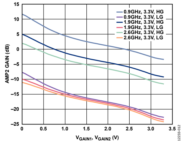
Figure 12. AMP2 Gain vs. V_{\text{GAIN1}} , V_{\text{GAIN2}} at Three Frequencies, 3.3 V Supply, Both Gain Controls Varied, V_{\text{GAIN1}} = V_{\text{GAIN2}}
