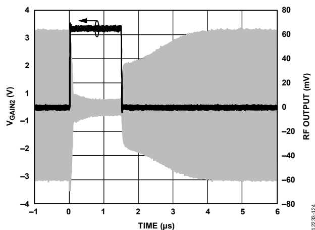
Figure 24. AMP2 Typical Output Response with 3.3 V Step on V_{\text{GAIN2}} , V_{\text{GAIN1}} = 0 \text{ V} , HG Mode, 0.9 GHz
