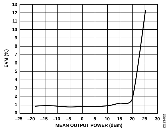
Figure 80. EVM vs. Mean Output Power ( P_{OUT} ) of Full Chain Connection at 2.2 GHz, 64 QAM, 5 MSPS, a = 0.2 Root Raised Cosine Filter, P_{IN} = -3.7 dBm
