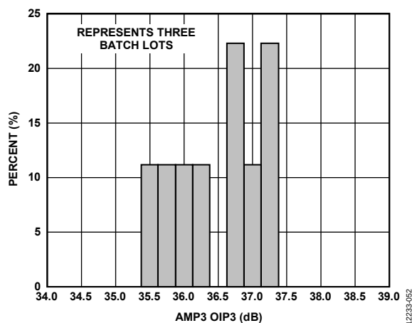
Figure 70. AMP3 OIP3 Distribution at 0 dBm/Tone, 2.2 GHz
