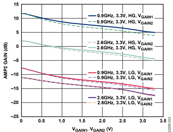
Figure 13. AMP2 Gain vs. V_{\text{GAIN1}} , V_{\text{GAIN2}} at Two Frequencies, 3.3 V Supply, Only One Gain Control Varied
