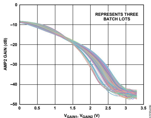
Figure 73. Distribution of AMP2 Gain vs. V_{GAIN1} , V_{GAIN2} at 1.5 GHz, 5 V Supply, LG, Both Gain Controls Varied, V_{GAIN1} = V_{GAIN2}
