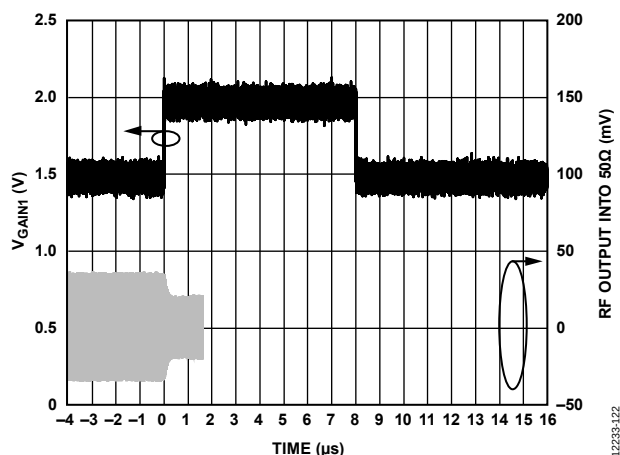
Figure 22. AMP2 Typical Output Response with 0.5 V Step on V_{\text{GAIN1}} , V_{\text{GAIN2}} = 0 \text{ V} , HG Mode, 0.9 GHz
