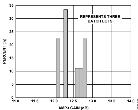
Figure 68. AMP3 Gain Distribution at 2.2 GHz
