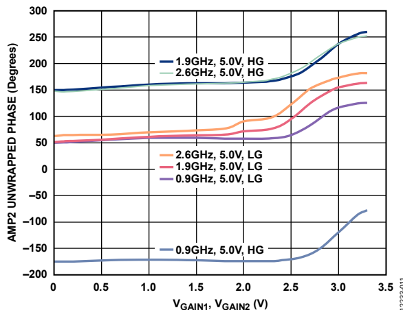
Figure 11. AMP2 Unwrapped Phase vs. V_{\text{GAIN1}} , V_{\text{GAIN2}} at Three Frequencies, 5 V Supply, Both Gain Controls Varied, V_{\text{GAIN1}} = V_{\text{GAIN2}}
