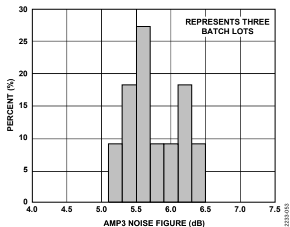
Figure 71. AMP3 Noise Figure Distribution, 2.2 GHz
