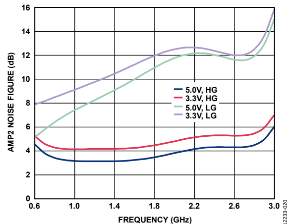
Figure 20. AMP2 Noise Figure vs. Frequency at V_{\text{GAIN1}} = V_{\text{GAIN2}} = 0 \text{ V}
