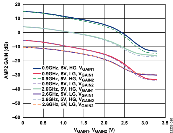
Figure 10. AMP2 Gain vs. V_{\text{GAIN1}} , V_{\text{GAIN2}} at Two Frequencies, 5 V Supply, Only One Gain Control Varied
