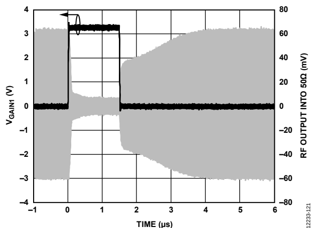
Figure 21. AMP2 Typical Output Response with 3.3 V Step on V_{\text{GAIN1}} , V_{\text{GAIN2}} = 0 \text{ V} , HG Mode, 0.9 GHz
