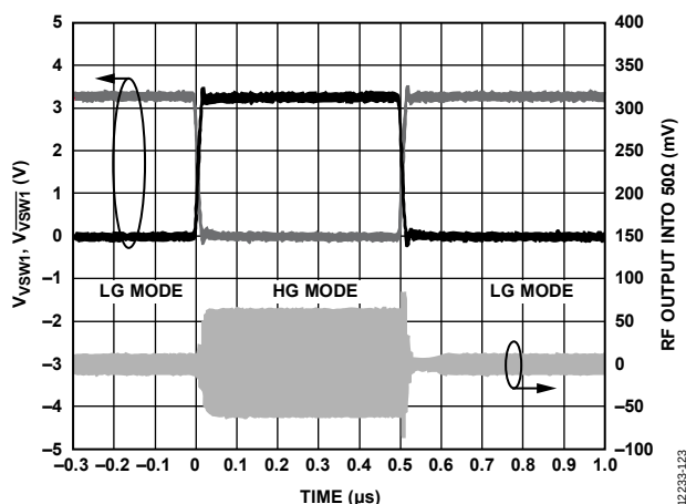
Figure 23. AMP2 Typical Output Response During Gain Mode Switching, V_{\text{GAIN1}} = V_{\text{GAIN2}} = 0 \text{ V} , 0.9 GHz
