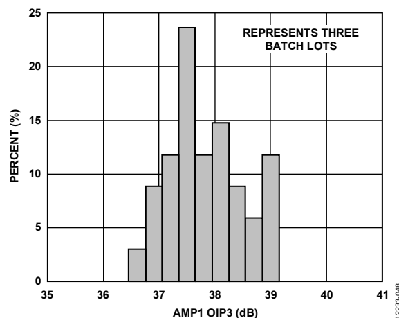
Figure 66. AMP1 OIP3 Distribution at 2.2 GHz, P_{OUT} = 0 dBm/Tone
