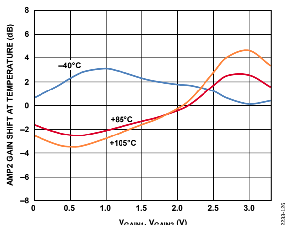
Figure 26. AMP2 Typical Gain Shift at Temperature With Respect to 25 °C vs. V_{\text{GAIN1}} = V_{\text{GAIN2}} , Both Gain Controls Varied, 1.75 GHz
