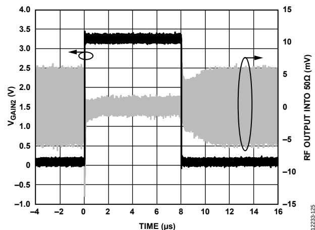
Figure 25. AMP2 Typical Output Response with 3.3 V Step on V_{\text{GAIN2}} , V_{\text{GAIN1}} = 3.3 \text{ V} , HG Mode, 0.9 GHz
