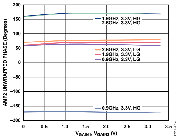
Figure 14. AMP2 Unwrapped Phase vs. V_{\text{GAIN1}} , V_{\text{GAIN2}} at Three Frequencies, 3.3 V Supply, Both Gain Controls Varied, V_{\text{GAIN1}} = V_{\text{GAIN2}}
