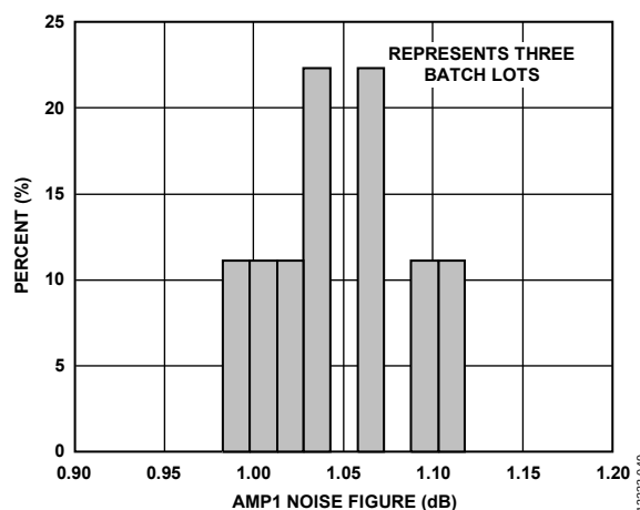
Figure 67. AMP1 Noise Figure Distribution at 2.2 GHz
