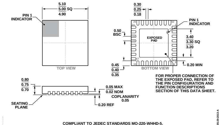
Figure 85. 32-Lead Lead Frame Chip Scale Package [LFCSP_WQ] 5 mm x 5 mm Body, Very Very Thin Quad (CP-32-20) Dimensions shown in millimeters
