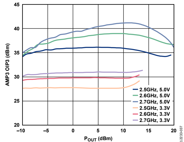
Figure 55. AMP3 2.6 GHz OIP3 vs. P_{OUT} by Frequency
