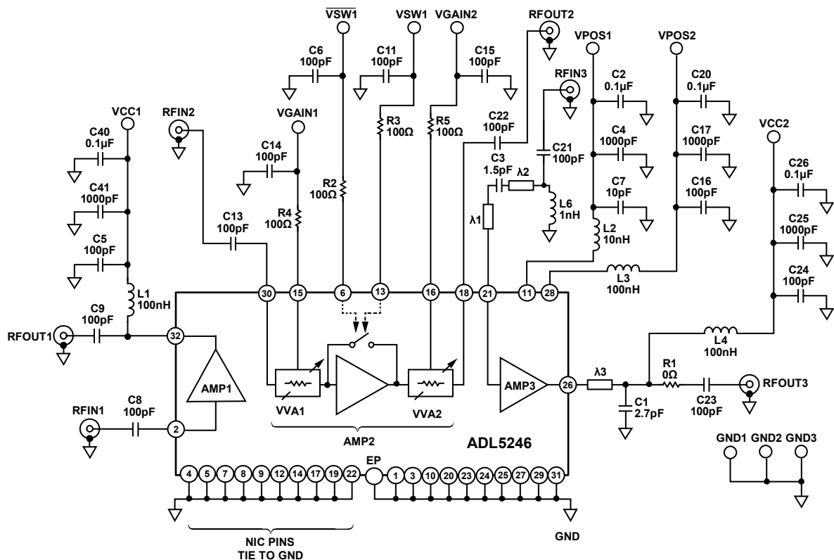
Figure 74. Basic Connections
