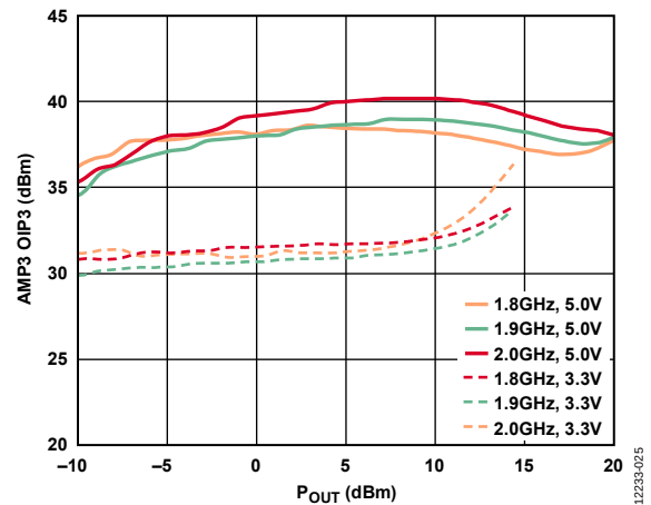
Figure 43. AMP3 1.9 GHz OIP3 vs. P_{OUT} by Frequency
