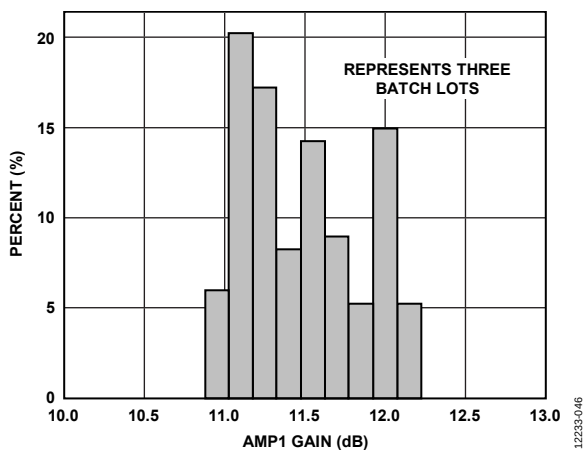
Figure 64. AMP1 Gain Distribution at 2.2 GHz
