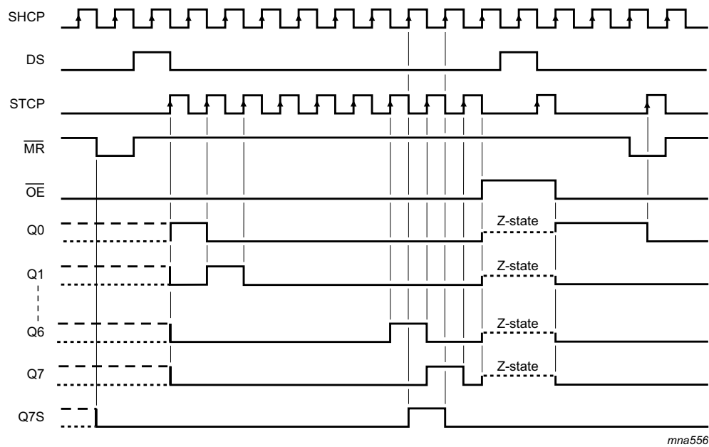
Fig 5. Timing diagram
