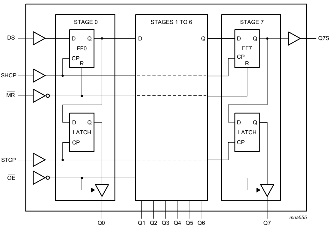
Fig 4. Logic diagram
