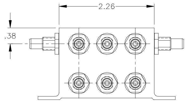
SIDE MOUNT BUS CONFIGURATION D-500-0255-562-1
