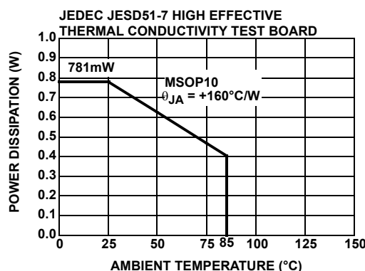
FIGURE 28. PACKAGE POWER DISSIPATION vs AMBIENT TEMPERATURE
