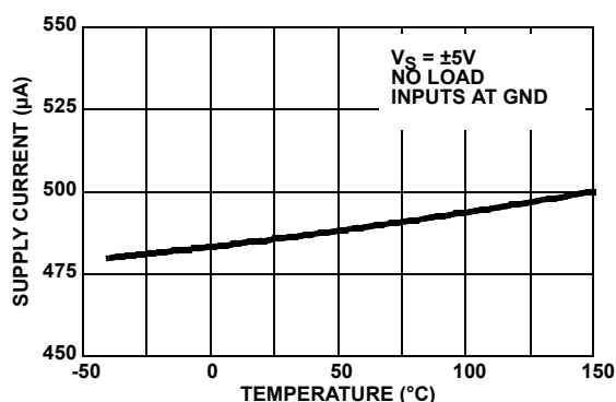
FIGURE 9. SUPPLY CURRENT PER CHANNEL vs TEMPERATURE
