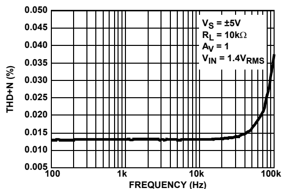
FIGURE 18. TOTAL HARMONIC DISTORTION + NOISE vs FREQUENCY
