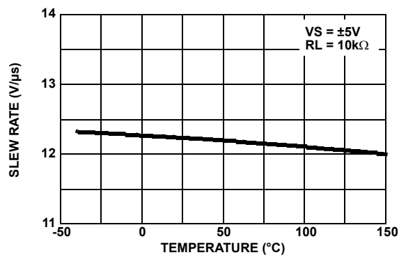
FIGURE 8. SLEW RATE vs TEMPERATURE
