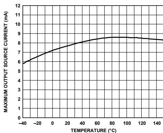
Figure 19. Maximum Output Source Current vs. Temperature Per Channel
