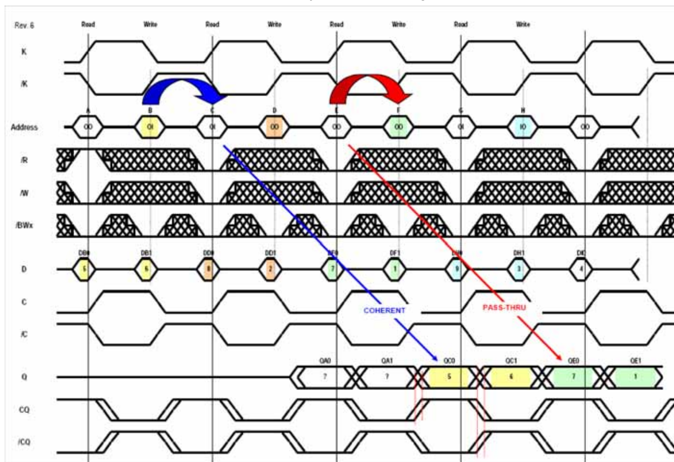
Burst of 2 Coherency and Pass Through Functions
