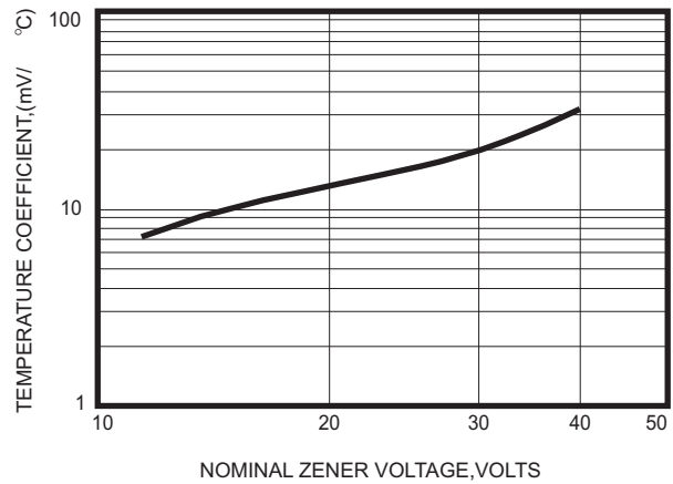
Fig.2 TEMPERATURE COEFFICENTS
