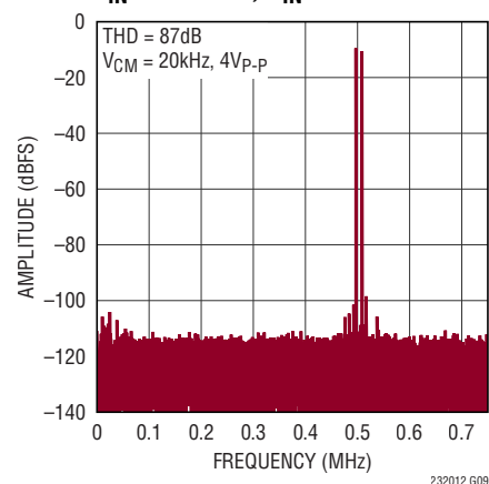
32k Point FFT, IMD, f_{\text{SMPL}} = 1.5\text{Mpsps} , A_{\text{IN}}^+ = 490\text{kHz} , A_{\text{IN}}^- = 510\text{kHz}
