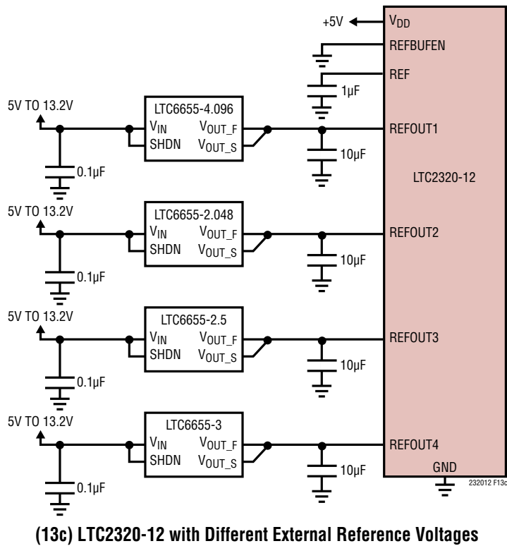
Figure 13. Reference Connections
