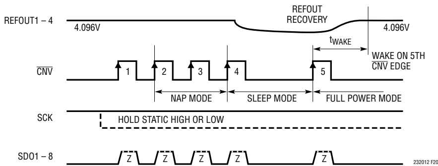
Figure 20. LVDS and CMOS Mode SLEEP and WAKE Using CNV
