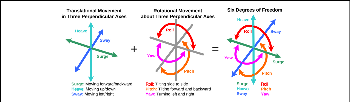
Figure 1. Six Degrees of Freedom General Definitions
