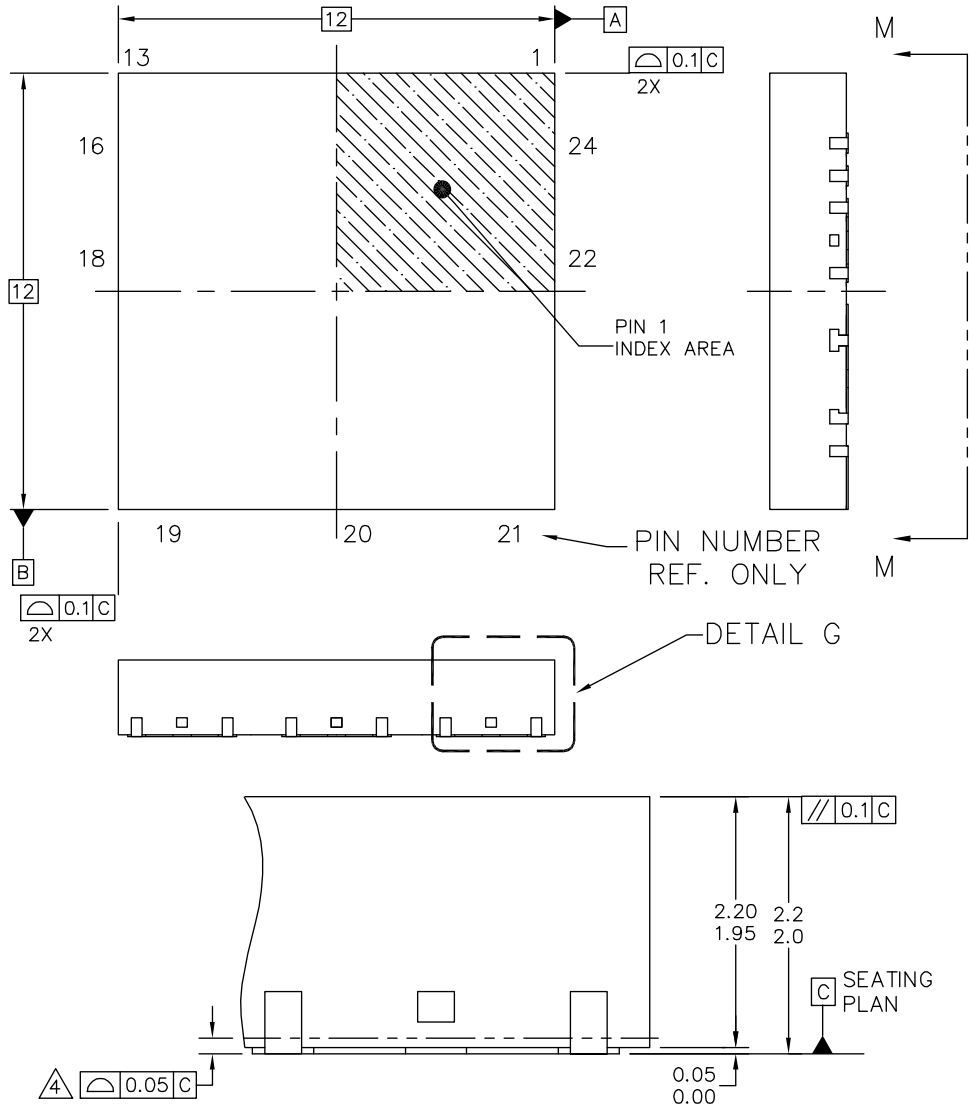
DETAIL G
