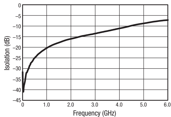
Figure 4. Isolation vs Frequency ( V_R = 0 V)
