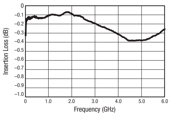
Figure 3. Insertion Loss vs Frequency ( I_f = 10 mA)
