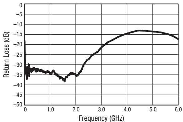
Figure 5. Return Loss vs Frequency ( I_f = 10 mA)
