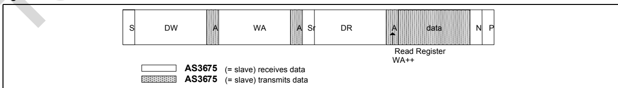
Figure 38. Serial Interface Random Read
