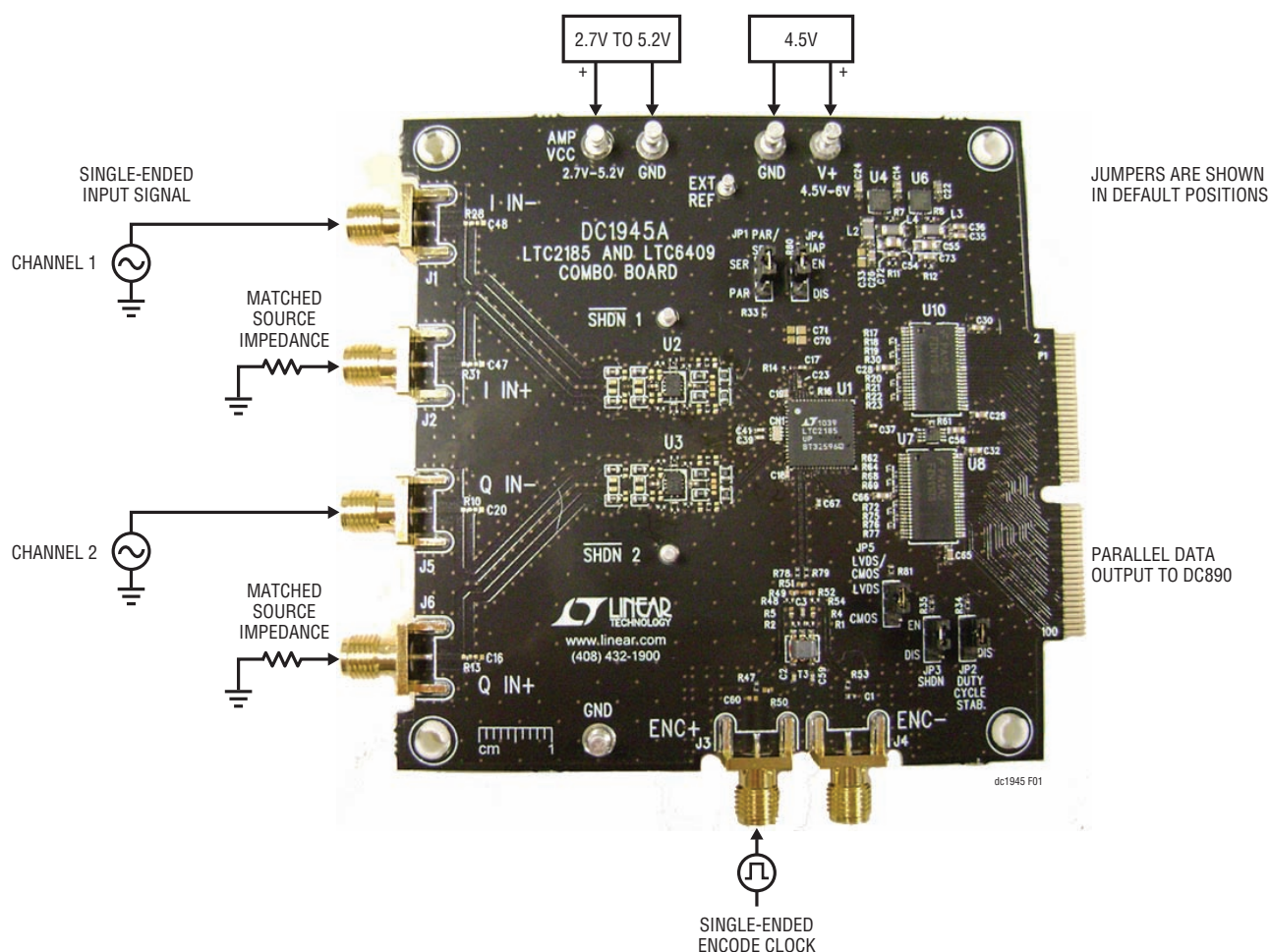
Figure 1. DC1945A Setup
