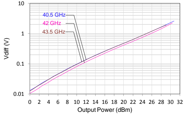
Power Detector vs. Pout vs. Frequency Vd = +6V, Id = 900 mA, Vg = -0.7 V Typical, 25°C
