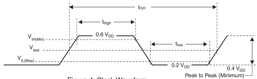
Figure 4. Clock Waveform
