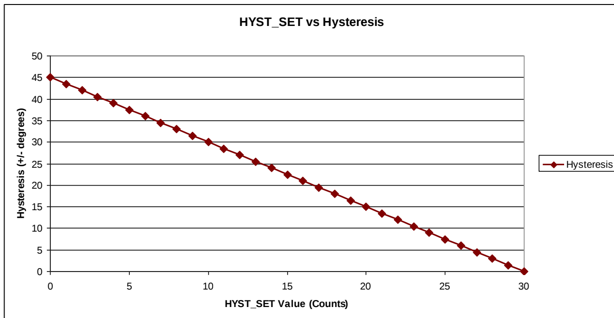
Figure 2. HYST_SET vs Hysteresis
