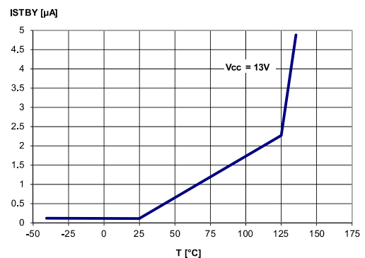
Figure 9: Standby current
