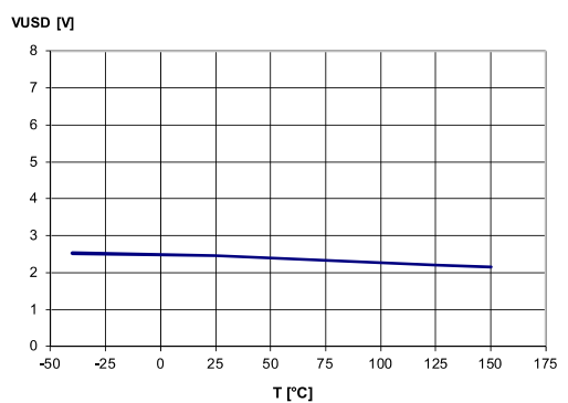
Figure 16: Undervoltage shutdown
