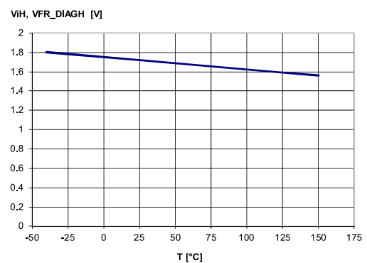
Figure 11: Logic input high level voltage
