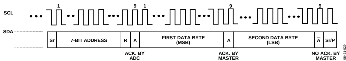
Figure 28. Mode of Operation, Single-Channel Conversion
