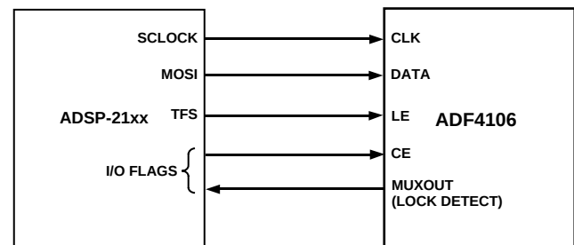
Figure 24. ADSP-21xx-to-ADF4106 Interface
