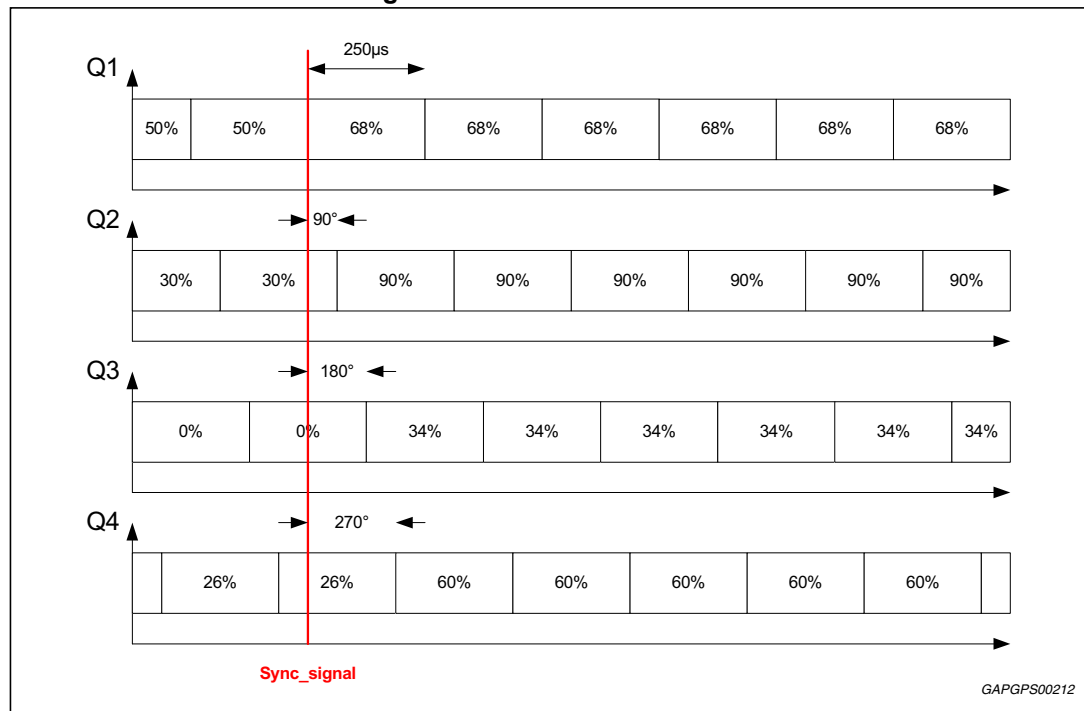
Figure 18. Channels time shift
