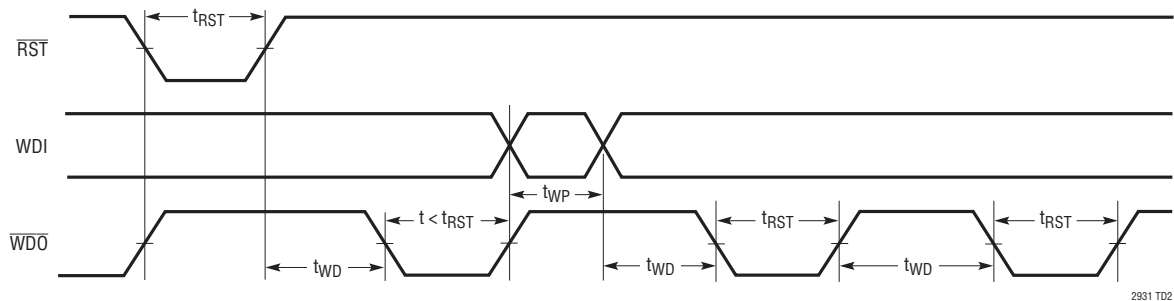
Watchdog Timing
