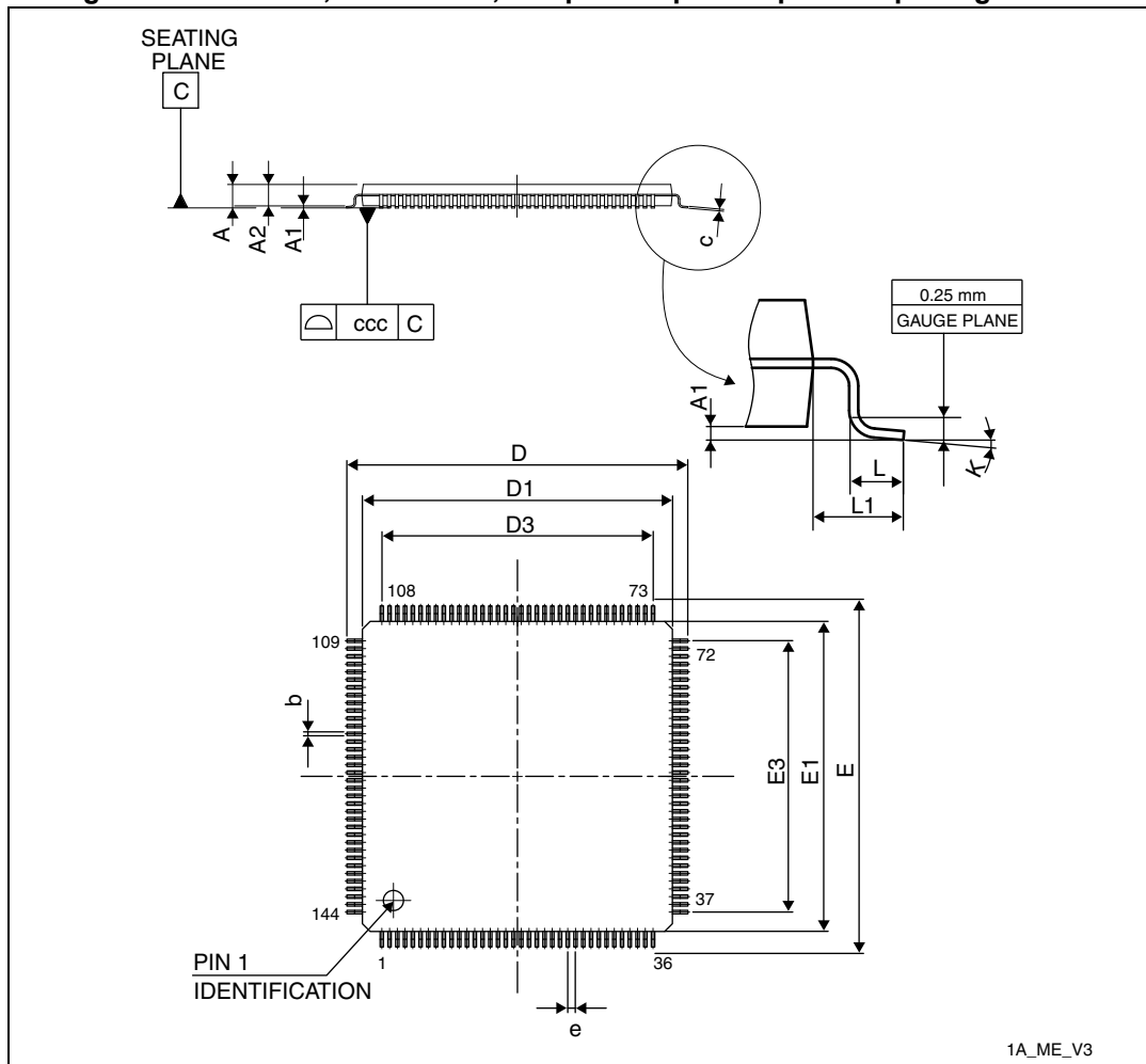
Figure 90. LQFP144, 20 x 20 mm, 144-pin low-profile quad flat package outline
