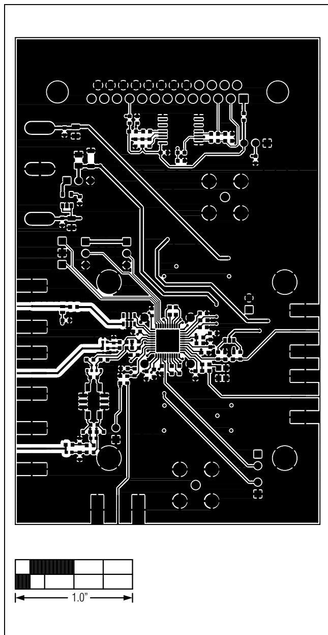
Figure 6. MAX2140 EV Kit PCB Layout—Component Side
