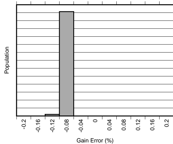
Figure 10. Gain Error Distribution (INA301A1)
