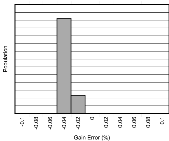
Figure 11. Gain Error Distribution (INA301A2)
