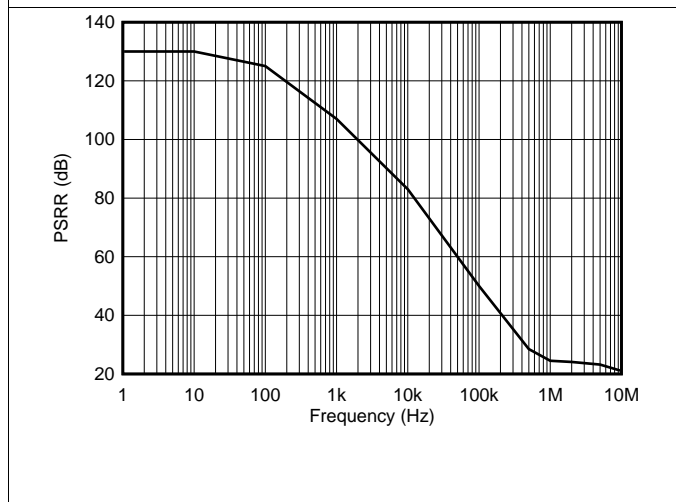
Figure 15. Power-Supply Rejection Ratio vs Frequency
