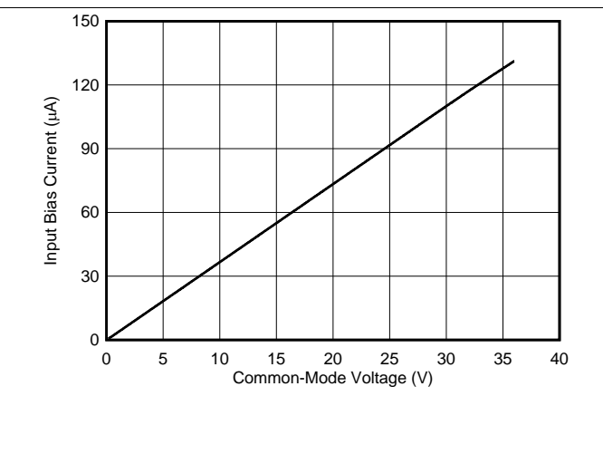
Figure 18. Input Bias Current vs Common-Mode Voltage ( V_S = 0\text{ V} )
