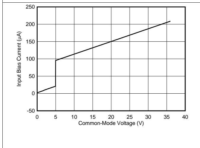
Figure 17. Input Bias Current vs Common-Mode Voltage ( V_S = 5\text{ V} )
