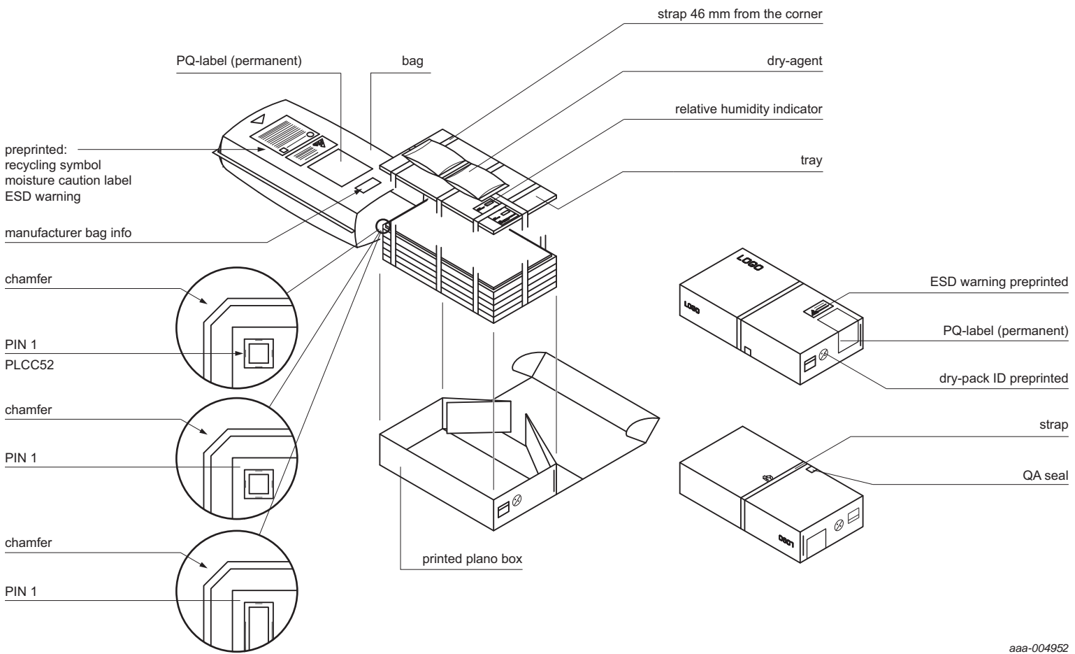
Fig 32. Packaging information 5 tray
