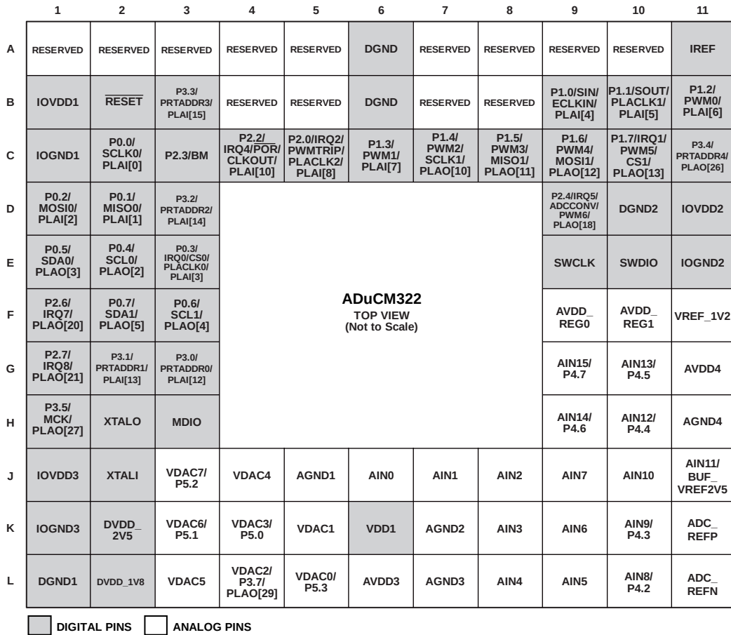
Figure 8. Pin Configuration
