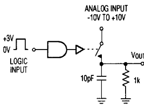
Figure 1. Switching Time
