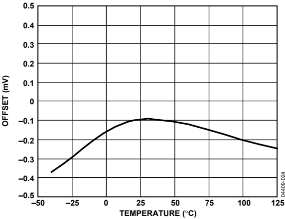
Figure 11. Input Offset Voltage vs. Temperature
