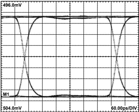
Figure 13. ADCMP572 Eye Diagram at 2.5 Gbps
