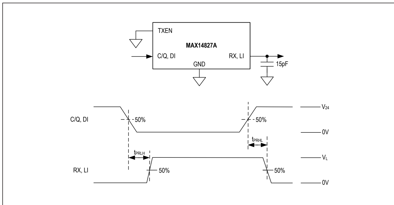
Figure 4. C/Q and DI Receiver Propagation Delays
