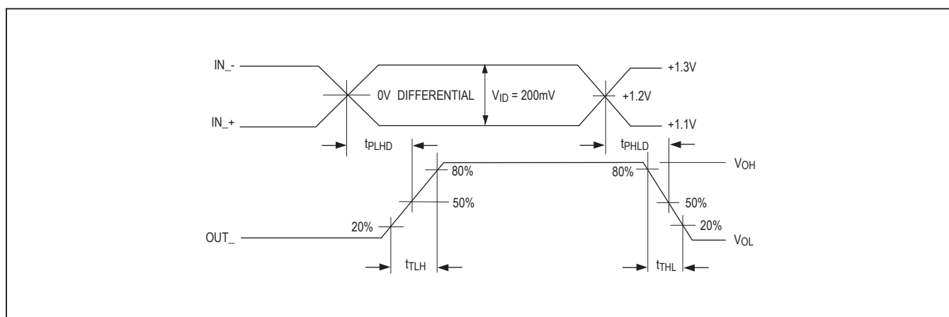
Figure 2. Receiver Propagation Delay and Transition Time Waveforms
